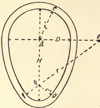
FIG. 2.—EGG-SHAPED SEWER.
